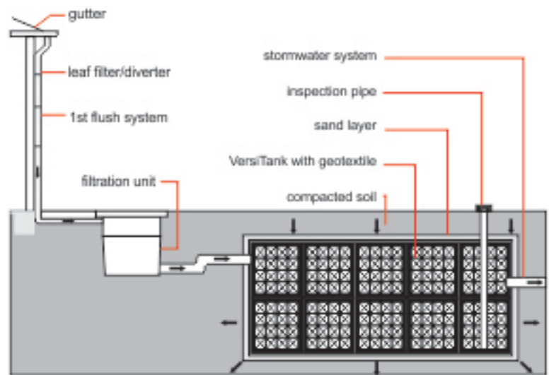
VersiTank Infiltration System
