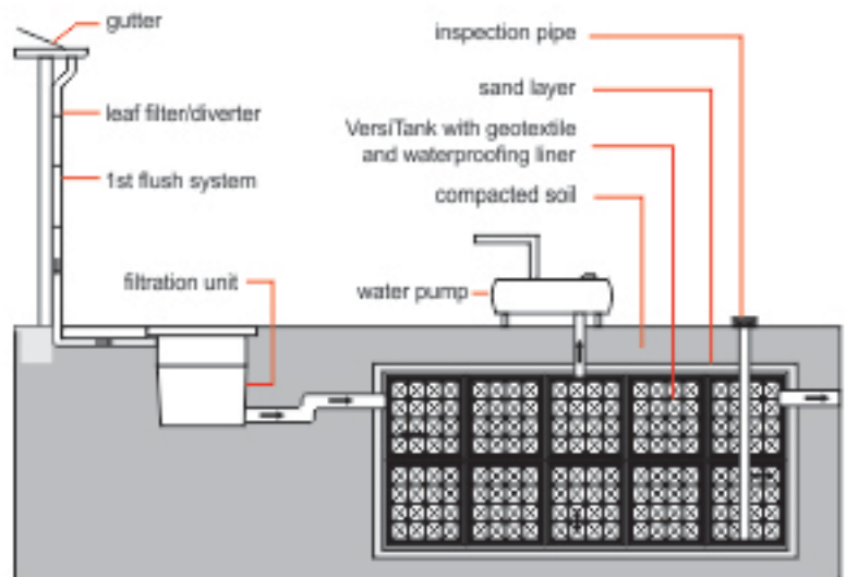
VersiTank Retention System
